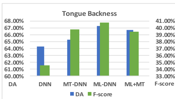
Figure 9: DA & F-score for tongue backness error.
