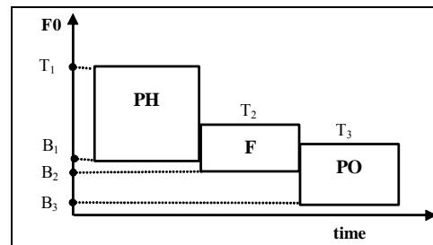
Figure 4: The envelope pattern definition for the F0 contour described by the functional sequence PH/F/PO
