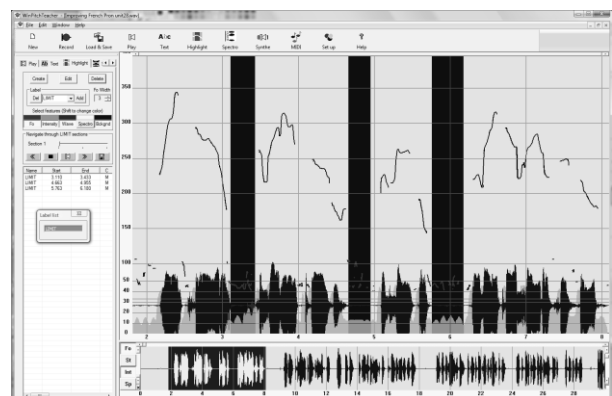
Fig. 6: Authoring program
