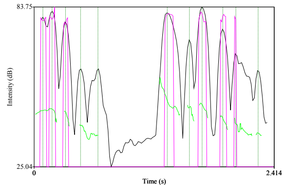
Figure 1: An energy profile (black) of a speech signal along with its pitch (green) and harmonicity (magenta) curves. Syllable nuclei are marked with dashed vertical lines.
