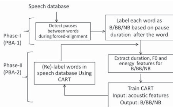
Figure 2: Flow chart of the proposed algorithm for learning speaker-specific phrase breaks.
