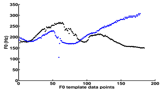
Figure 1: F0 values for a statement/question pair with stress pattern 10010.
