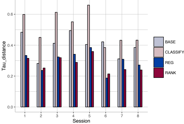
Figure 3: Performances of SI models over sessions.
