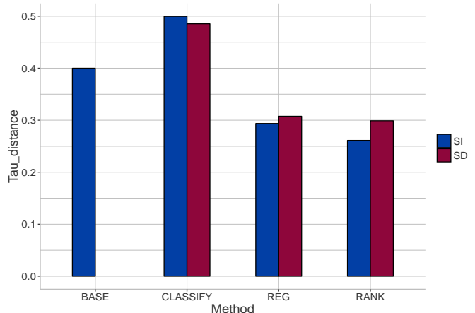
Figure 2: Overall performances of the methods.
