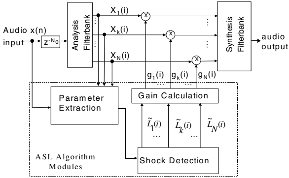
Figure 1: Acoustic-shock limiting (ASL) system.
