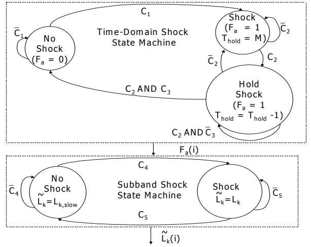
Figure 2: Shock detection state machines.
