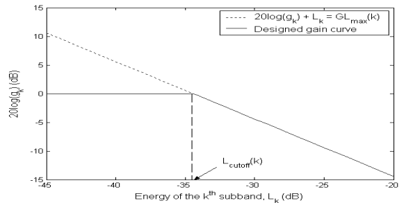
Figure 4: Design of input-gain (IG) curve.
