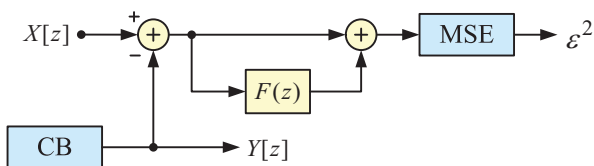
Figure 4: G.711.1 core layer using a VQ codebook
