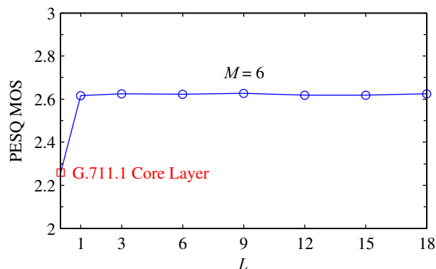
Figure 6: PESQ MOS as a function of L for an attenuation of 40 dB. The first point is for the G.711.1 core layer.
