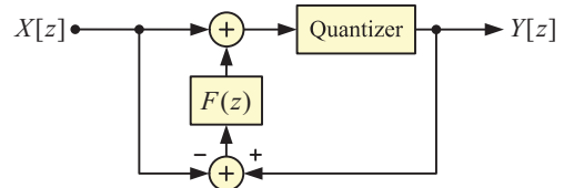
Figure 1: Noise shaping quantizer
