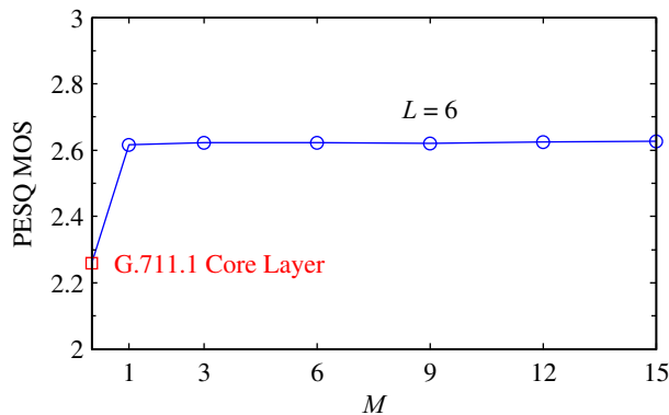
Figure 5: PESQ MOS as a function of M for an attenuation of 40 dB. The first point is for the G.711.1 core layer.
