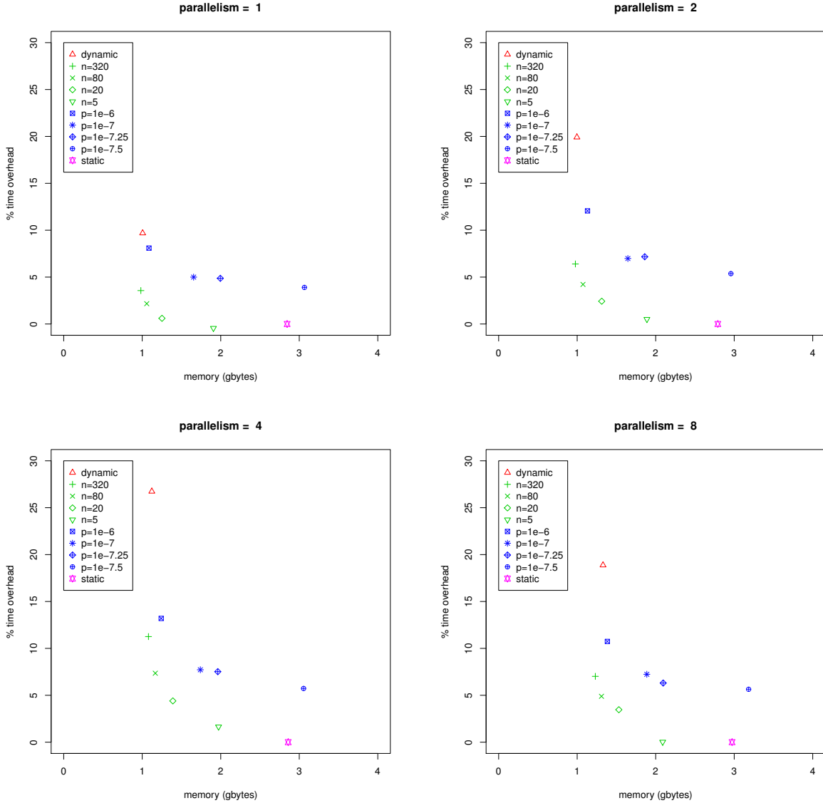
Figure 2: Total CPU memory usage (RAM) versus percent total recognition time in excess of that with fully-static composition with the same 1000 utterances served from one, two, four and eight threads for various recognition transducer expansion methods. The magenta six-sided star shows fully static case, the red triangle shows the fully-dynamic case, the blue points show the statistics-based method for various count cutoffs and the green points show the the probability-based method for various probability cutoffs.
