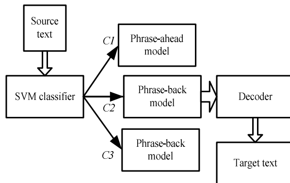
Figure 2: Architecture of Bandore.
