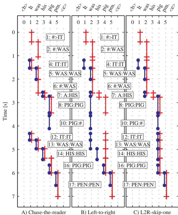
Figure 2: Comparing time-aligned ART traces (red plus-capped lines) with time-aligned reference traces (blue circle-capped lines). Spoken: “it was a pig pig it was his pig pen”, recognized: “it was it was was his pig it was his pig pen”.
