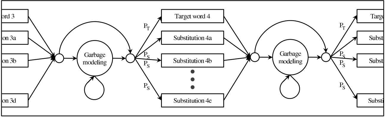
Figure 1: A part of the specialized language model centered on the fourth target word, which in this case has 5 (a,b, ... , e) optional substitutions. P_T is the probability of the target word, P_S is the probability of a substitution.
