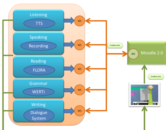
Figure 1: Architecture of the virtual environment
