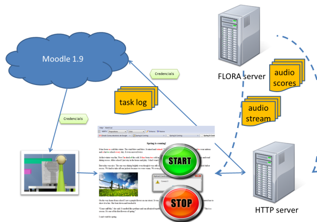
Figure 2: Architecture of the reading task
